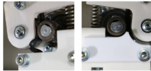
Flexible filament bending and twisting without and extruding smoothly with the adapter installed.
