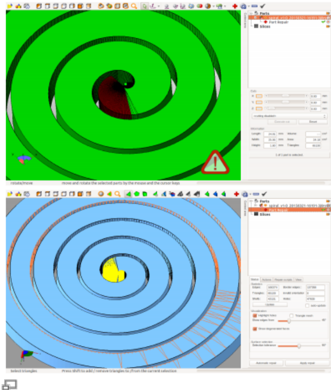
Alert of mismatches in an STL and the preview of misaligned edges and holes in netfabb basic's part repair.
