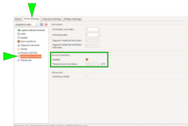
Ooze prevention selection in the “Print Settings” tab of Slic3r.
