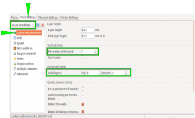
Load the calibration cube stl-file in Slic3r.
