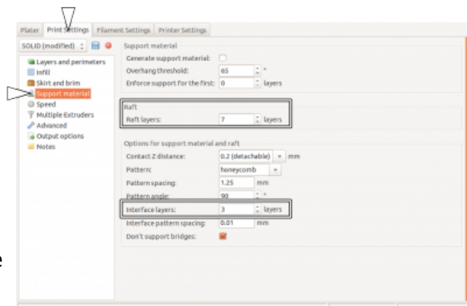
Adding a freely chosen number of raft layers to the print.
