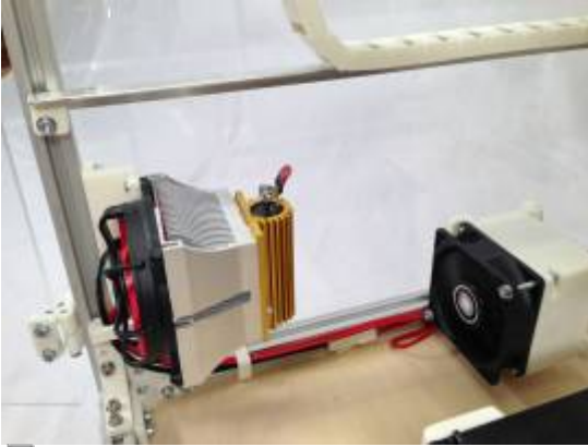
One of four circulating air heaters - each providing 120W for 70°C chamber temperature
