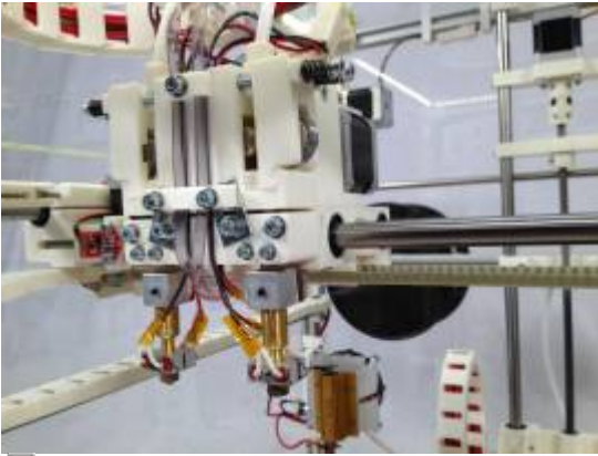
Dual extruders, front view - water cooled hotend insulators
