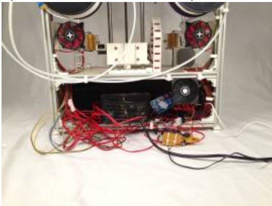
Back view - cable harness waiting for new high power MOSFET driver boards to be finally wired up
