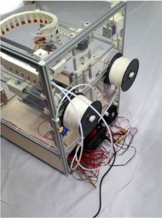
Spool holders on the back - plus cable mania..
