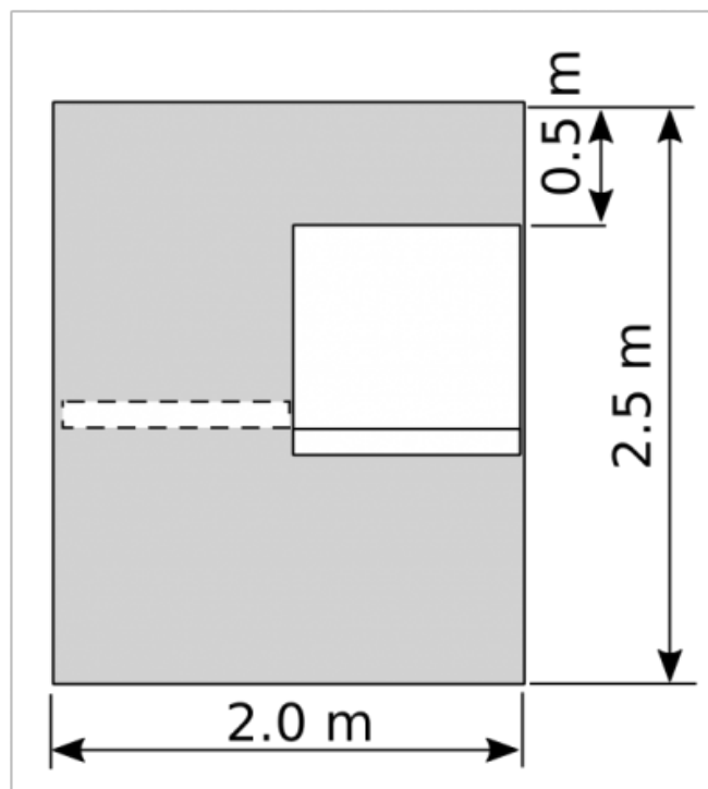
Necessary free space around the VP75.
